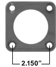
Greddy 47 mm
