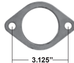
Counterbored for 2.125" O.D.tube
