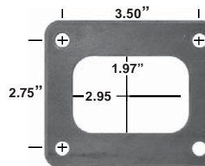
T04E (Wide Bolt Pattern)
